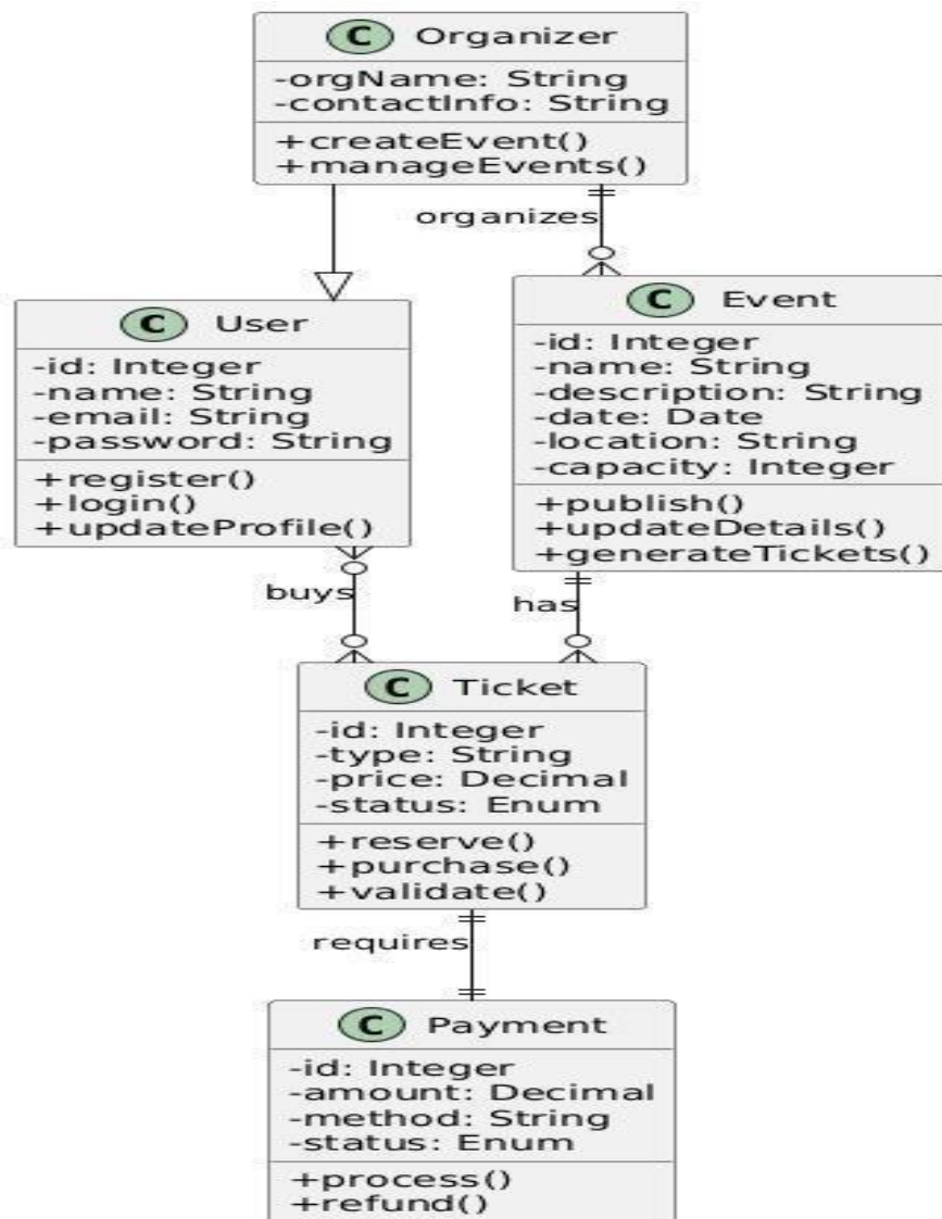
UML Class Diagram
