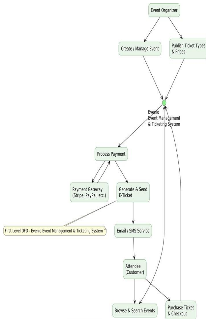
Figure 8: Data Flow Diagram
