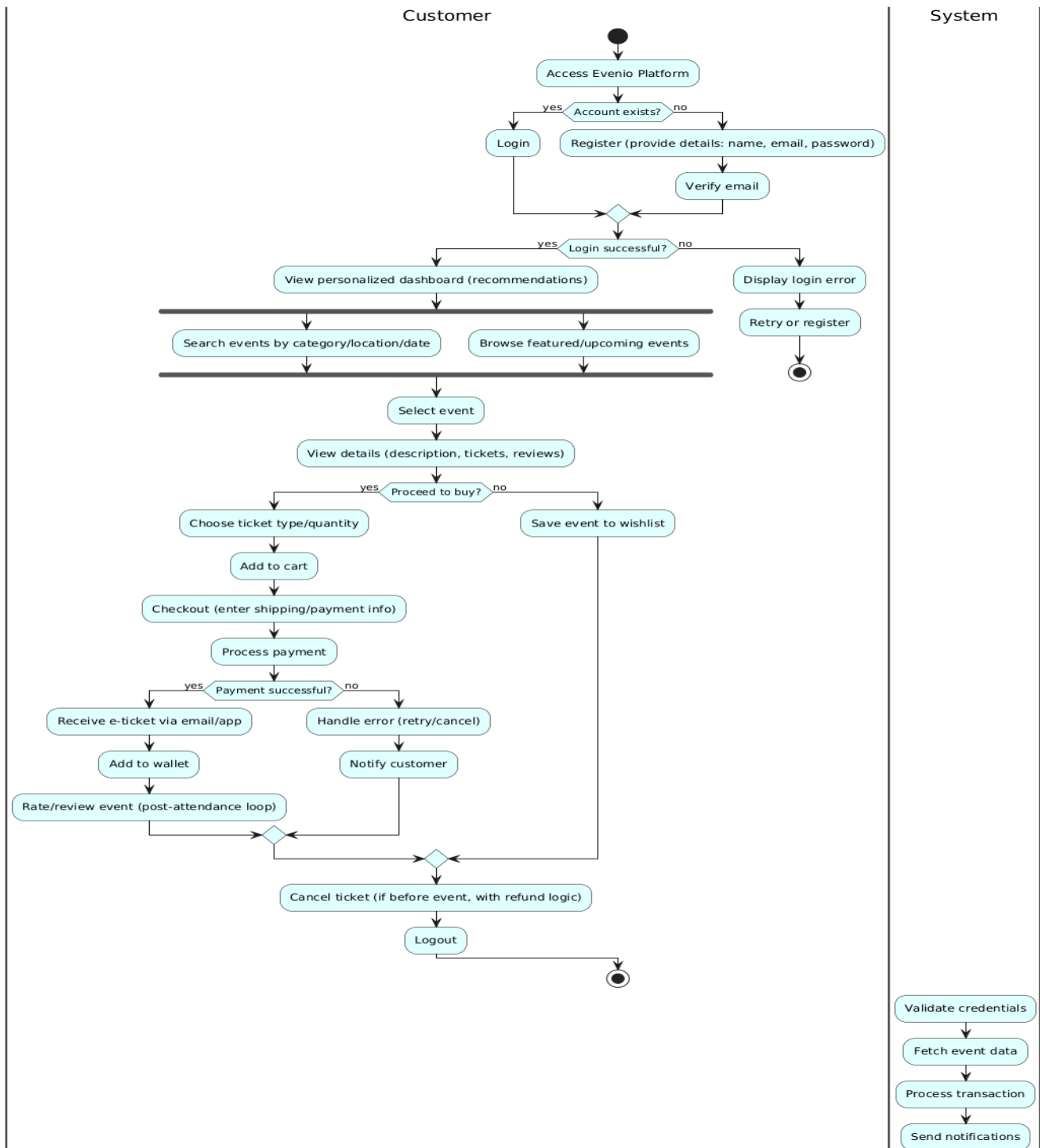
Figure 6:Customer Activity Diagram
