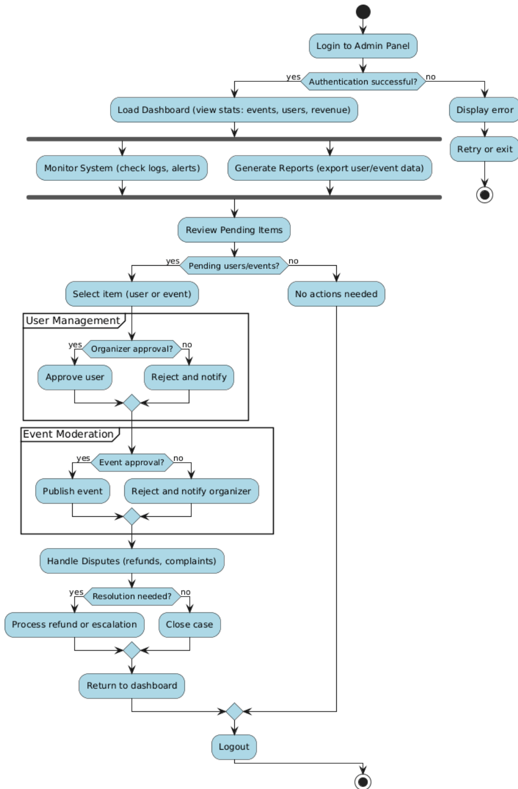
Figure5:Admin Activity Diagram
